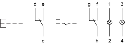
18 Illuminated pushbutton actuator two-part page 9
