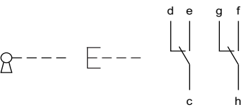
19 Keylock switch actuator 2 positions page 11 | Mushroom-head keylock switch 2 positions page 12
