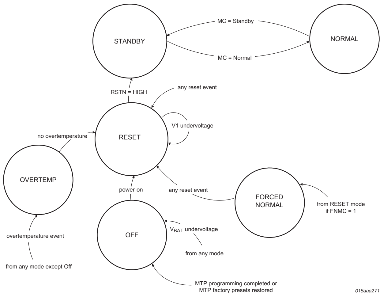
Fig 3. UJA1164 system controller state diagram
