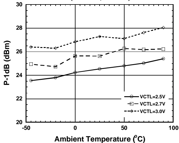
PC-P1 P-1dB vs. Ambient Temperature
