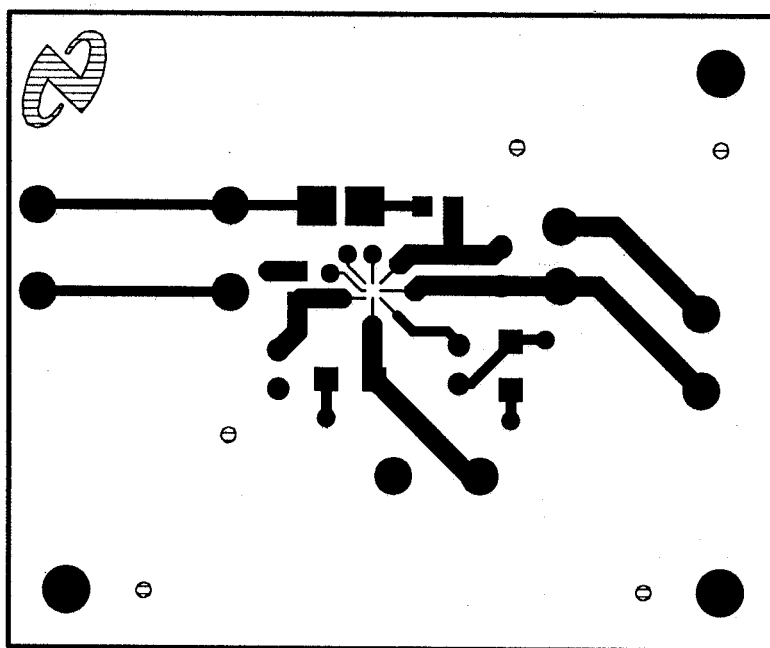
Figure 41. Top Layer
