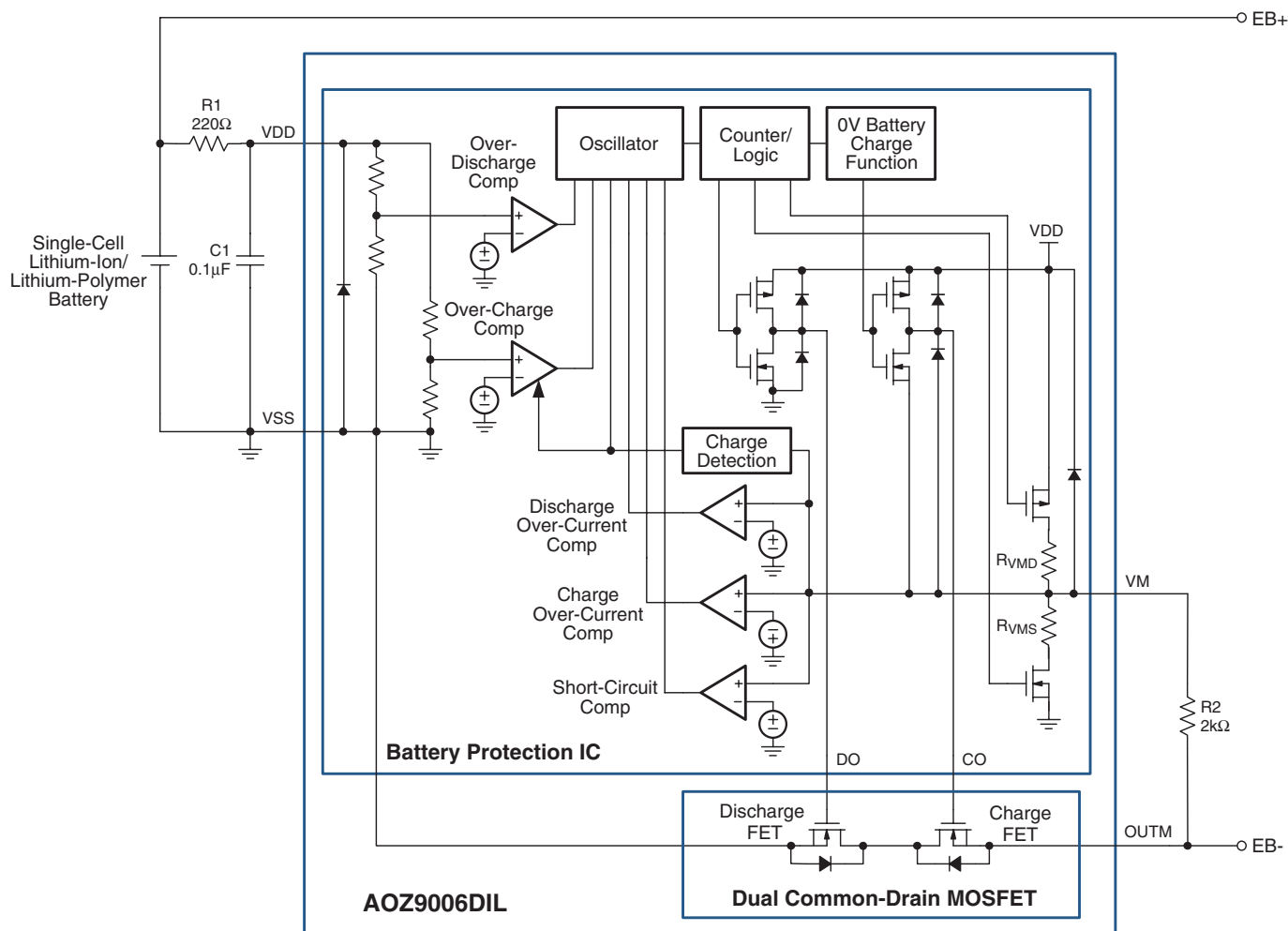
Figure 1. AOZ9006DIL Function Block Diagram
