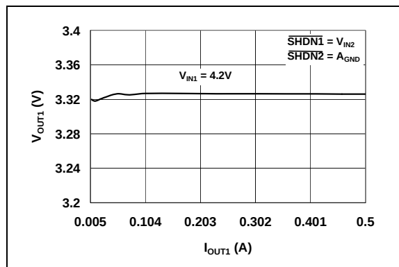
FIGURE 2-12: V_{OUT1} vs. I_{OUT1} ( V_{OUT1} = 3.3V ).
