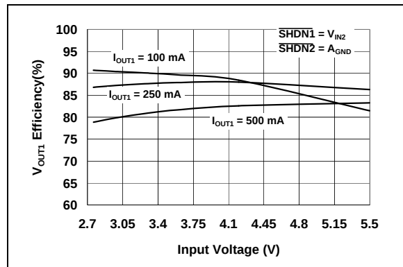
FIGURE 2-6: V_{OUT1} Output Efficiency vs. Input Voltage ( V_{OUT1} = 1.8V ).
