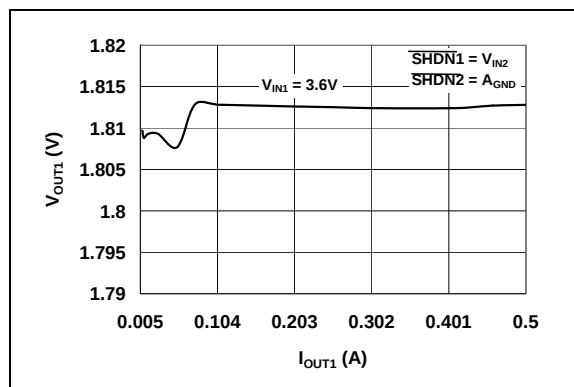
FIGURE 2-11: V_{OUT1} vs. I_{OUT1} ( V_{OUT1} = 1.8V ).
