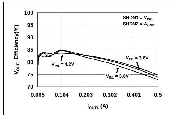
FIGURE 2-5: V_{OUT1} Output Efficiency vs. I_{OUT1} ( V_{OUT1} = 1.2V ).
