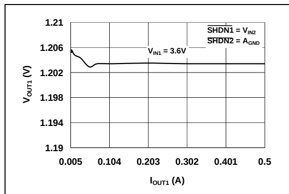
FIGURE 2-10: V_{OUT1} vs. I_{OUT1} ( V_{OUT1} = 1.2V ).
