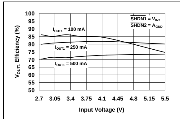
FIGURE 2-4: V_{OUT1} Output Efficiency vs. Input Voltage ( V_{OUT1} = 1.2V ).
