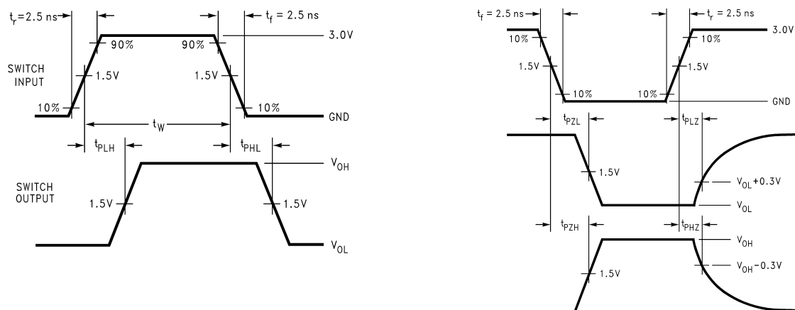
FIGURE 2. AC Waveforms
