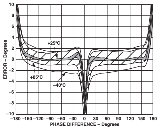
TPC 30. Distribution of VPHS Error vs. Input Phase Difference, Three Sigma to Either Side of Mean, Frequency 900 MHz, -40°C, +25°C, and +85°C, Input Levels -30 dBm
