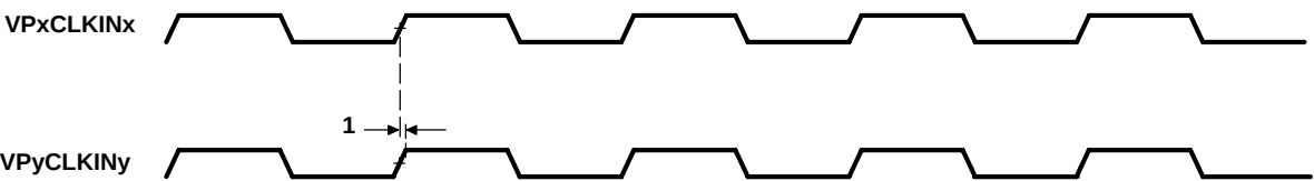
Figure 4–54. Video Port Dual-Display Sync Timing
