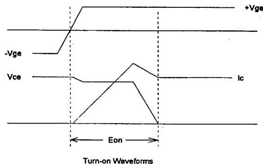
Switching waveforms
