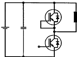
Test Circuit
