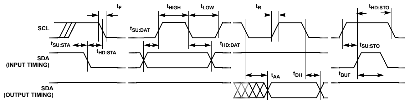
FIGURE 1. BUS TIMING
