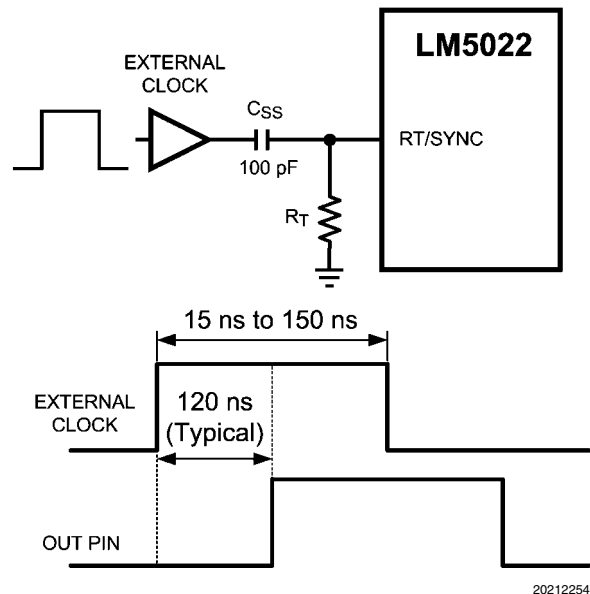
FIGURE 3. Sync Operation
