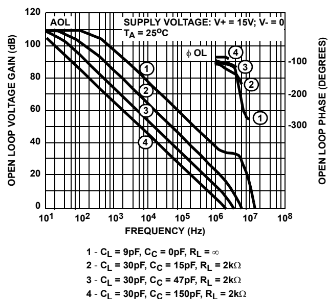
FIGURE 19. OPEN-LOOP RESPONSE
