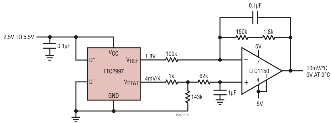
Figure 15. Celsius Thermometer
