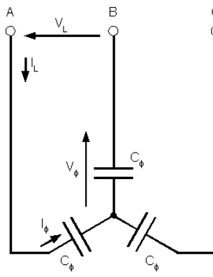
Wye Connection
