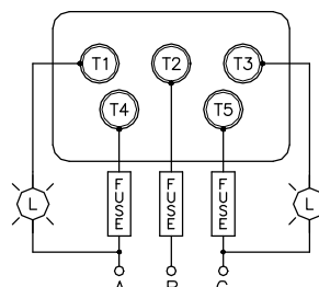
Figure 3: External Connections for Loss-of-kVAR Option
