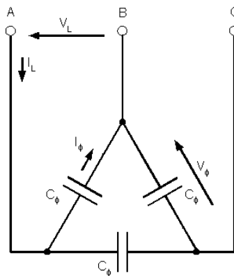
Delta Connection
