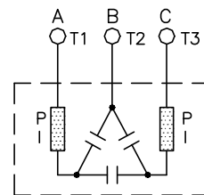
Figure 1: Internal Schematics for Low Voltage Three-Terminal Capacitors
