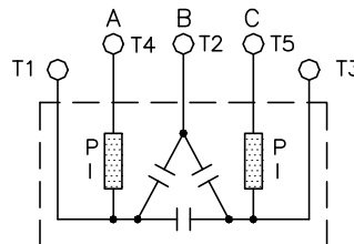
Figure 2: Internal Schematics for Five-Terminal Capacitors
