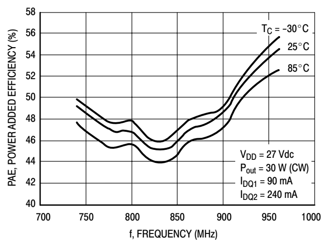
Figure 12. Power Added Efficiency versus Frequency
