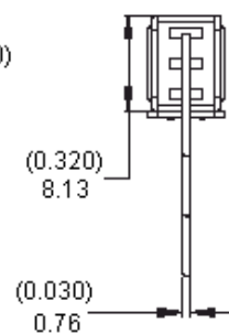
Section A - A Terminal Numbers for Reference Only
