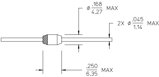
DIODE DIMENSION LIMITATIONS
