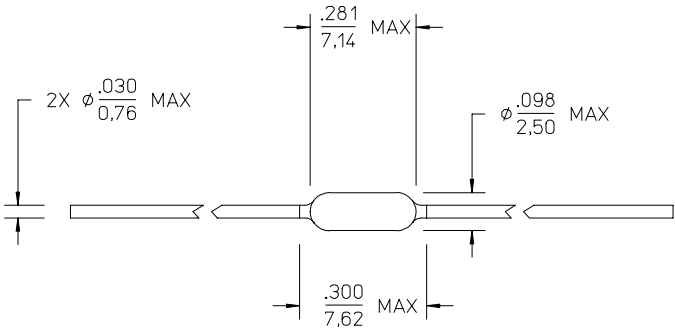
RESISTOR DIMENSION LIMITATIONS
