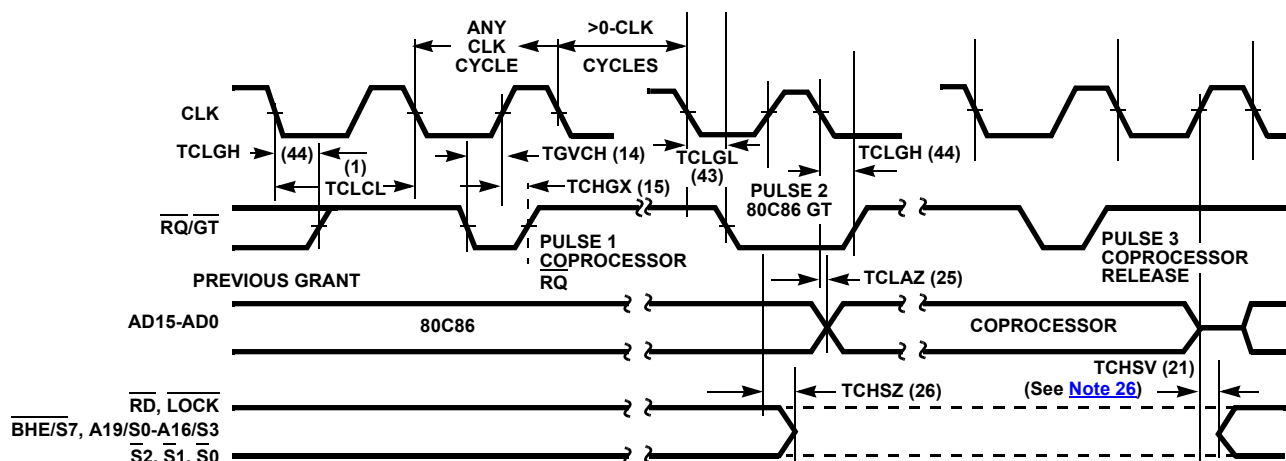
FIGURE 10. REQUEST/GRANT SEQUENCE TIMING (MAXIMUM MODE ONLY)
