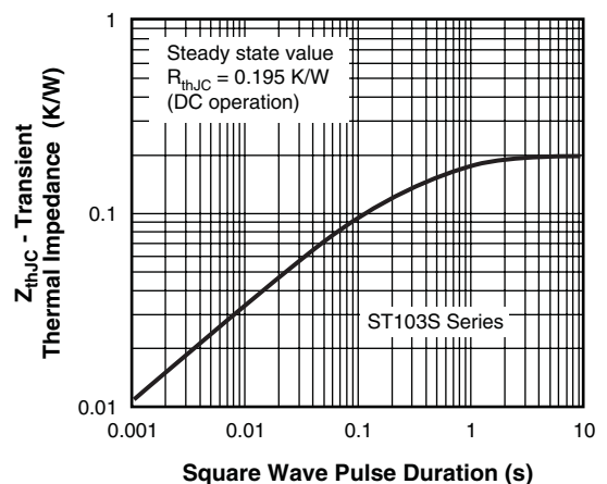
Fig. 8 - Thermal Impedance Z_{thJC} Characteristic
