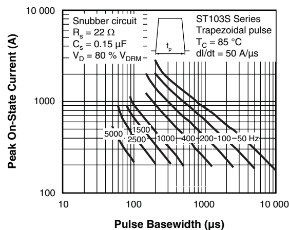
Fig. 12 - Frequency Characteristics
