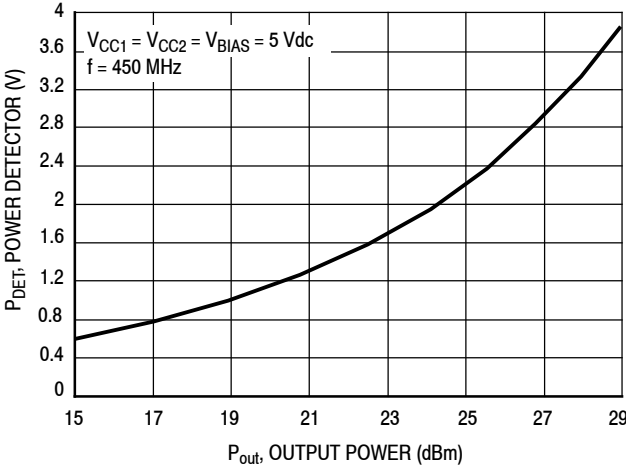
Figure 44. Power Detector versus Output Power, CW
