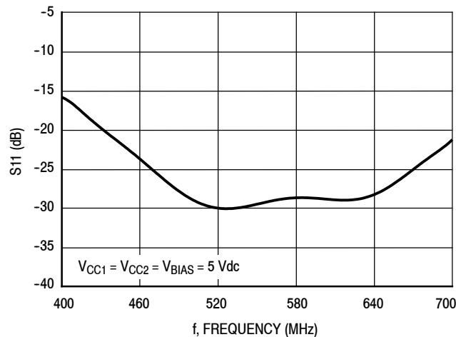
Figure 39. S11 versus Frequency
