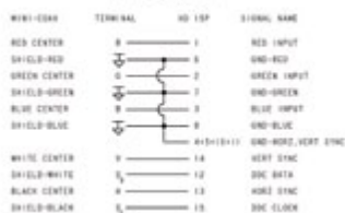
WIRING DIAGRAM
