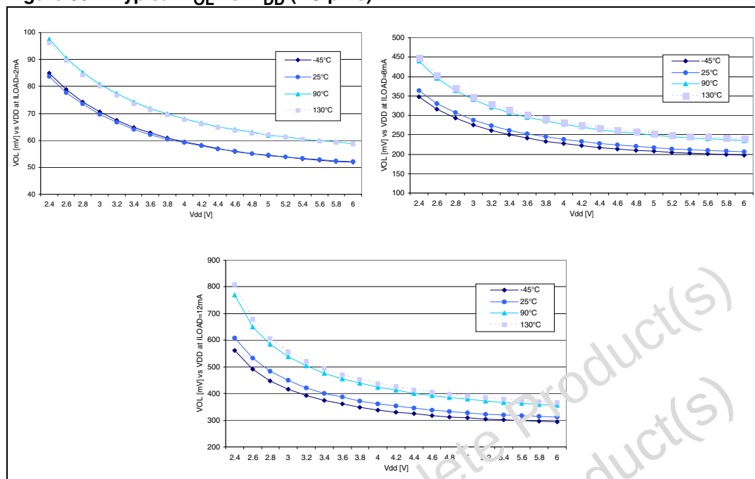
Figure 59. Typical V_{OL} vs. V_{DD} (HS pins)
