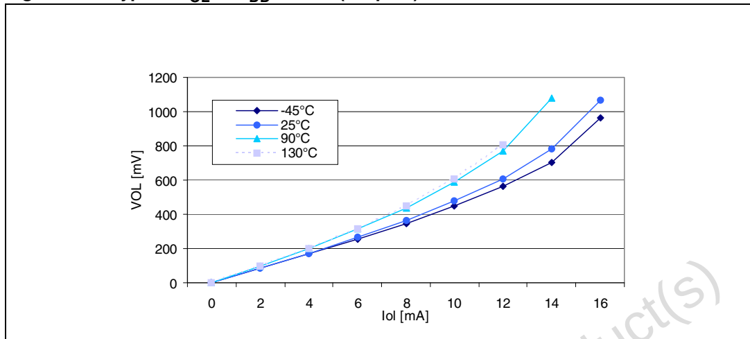
Figure 53. Typical V_{OL} at V_{DD} = 2.4 V (HS pins)
