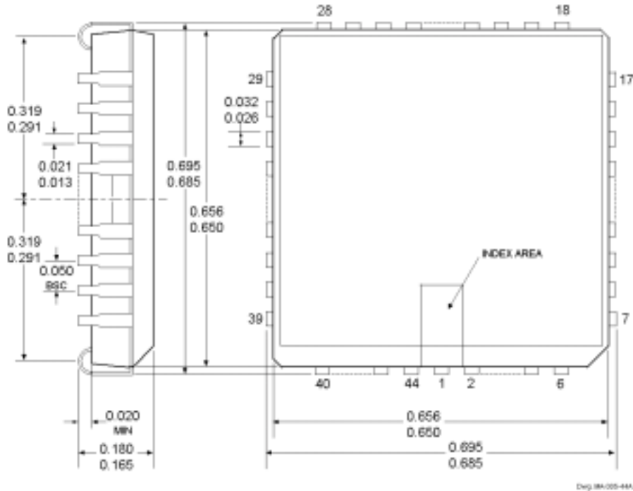
A3935KED (PLCC)
