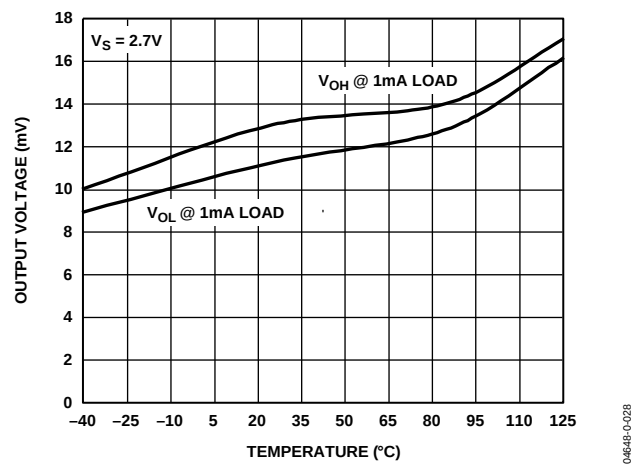
Figure 30. Output Voltage Swing vs. Temperature
