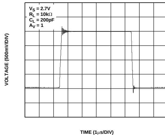
Figure 37. Large-Signal Transient Response
