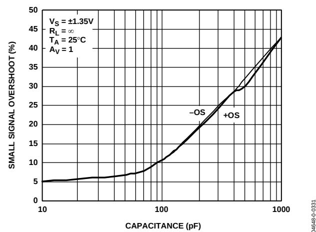
Figure 33. Small-Signal Overshoot vs. Load Capacitance
