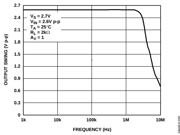
Figure 32. Closed-Loop Output Voltage Swing vs. Frequency
