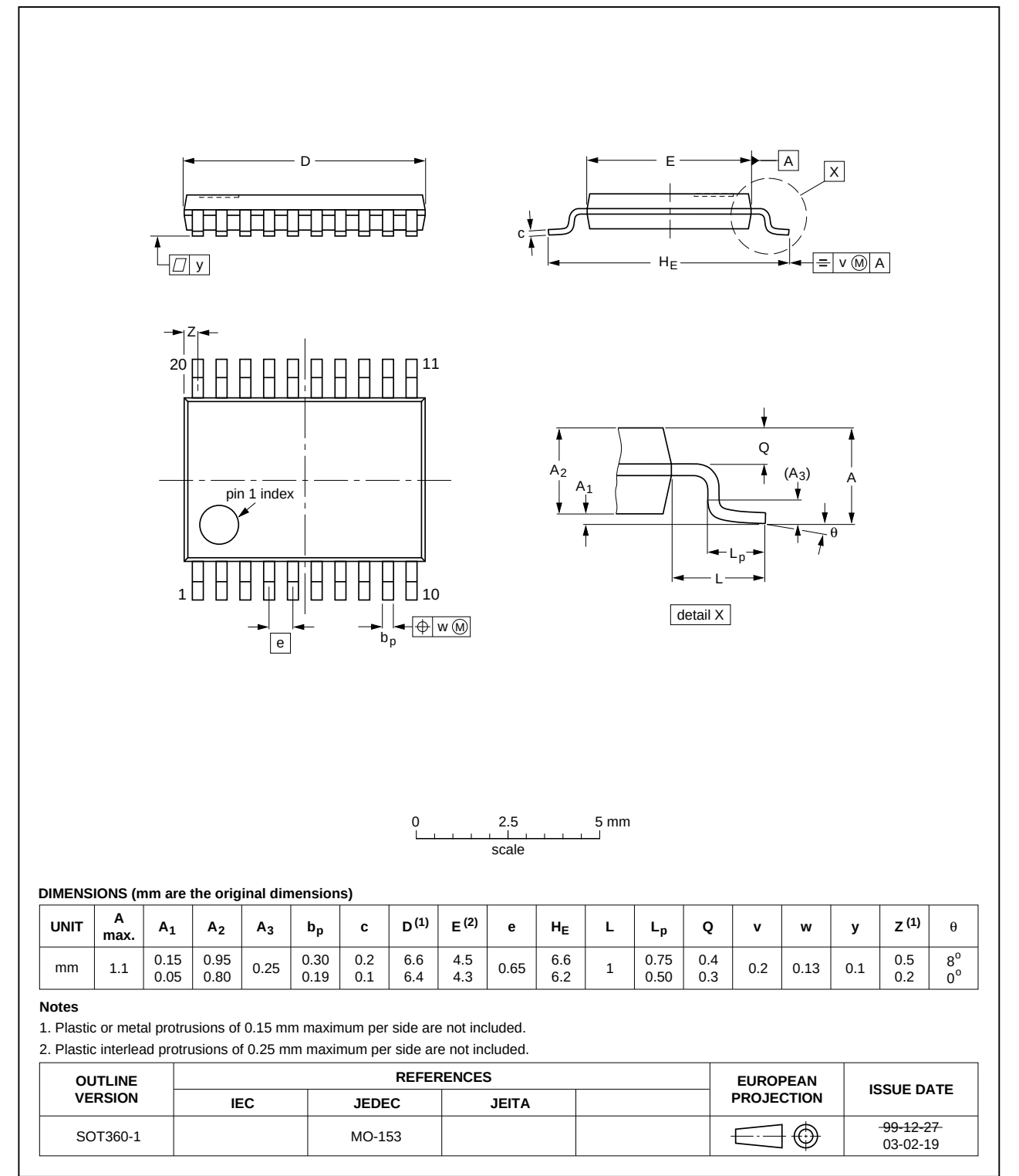
Fig 55. Package outline SOT360-1 (TSSOP20)
