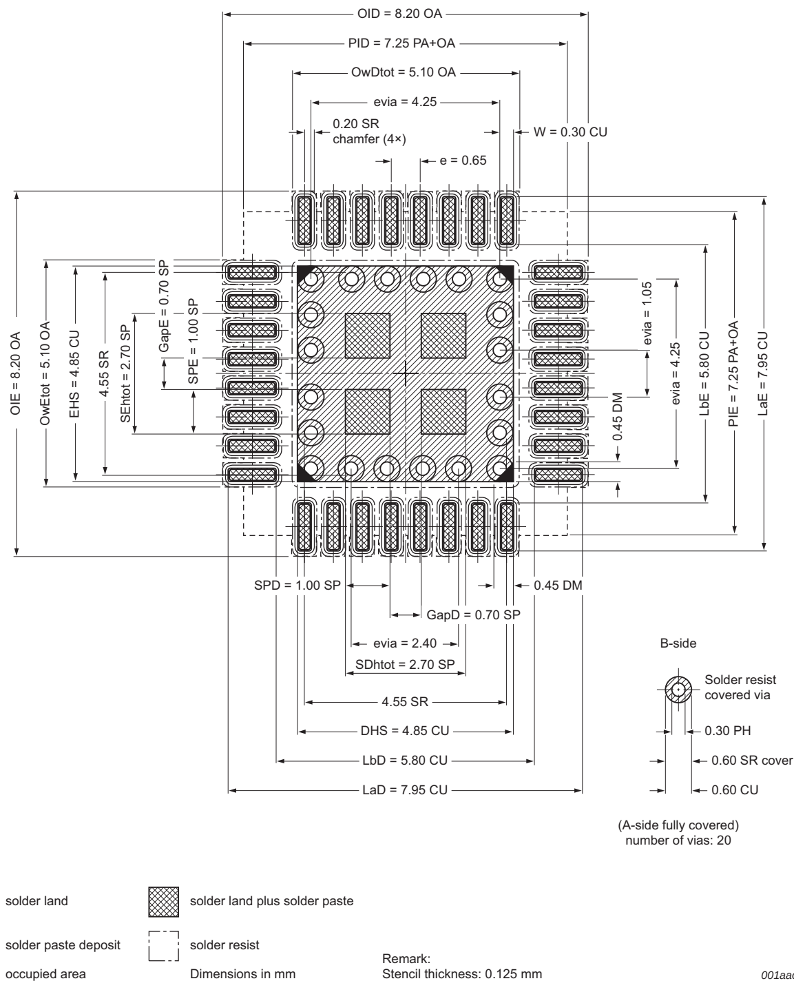
Fig 68. Reflow soldering of the HVQFN33 package (7x7)
