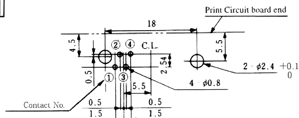
PCB mounting hole layout (Connector mounting side)
