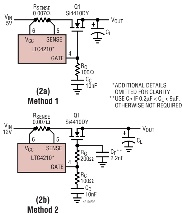
Figure 2. Frequency Compensation
