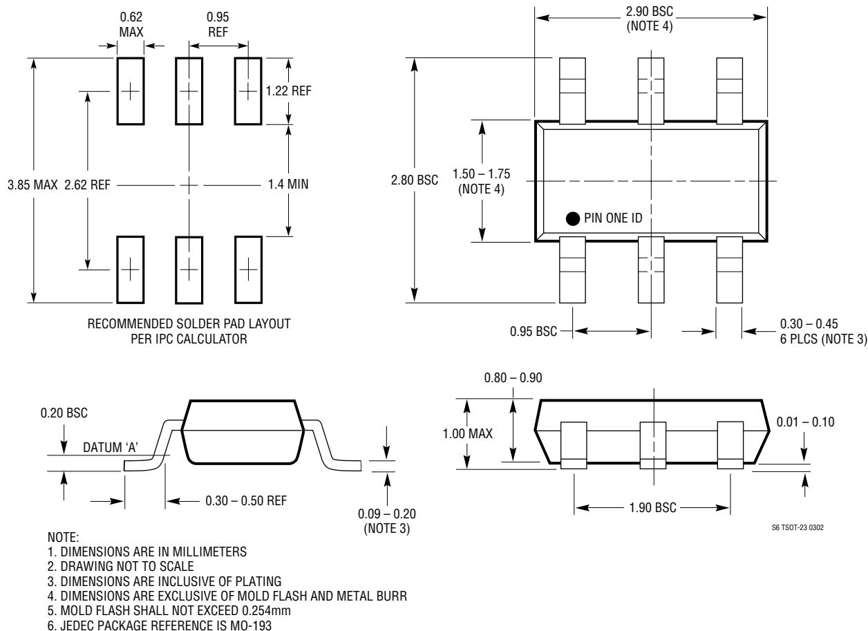
S6 Package 6-Lead Plastic TSOT-23 (Reference LTC DWG # 05-08-1636)
