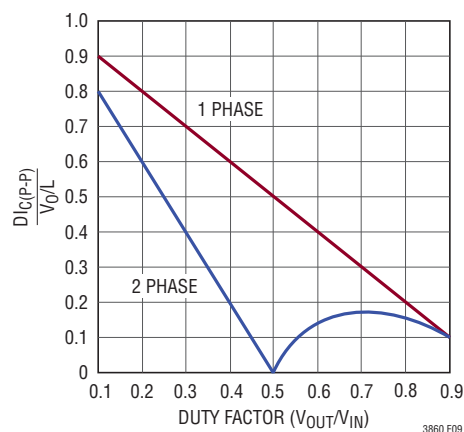
Figure 9. Normalized Output Ripple Current vs Duty Factor [ I_{RMS} = 0.3 (D I_C(P-P)) ]
