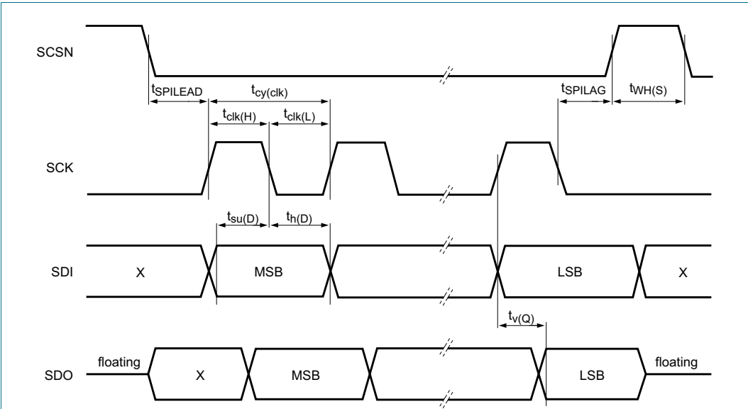
Fig 15. SPI timing diagram
