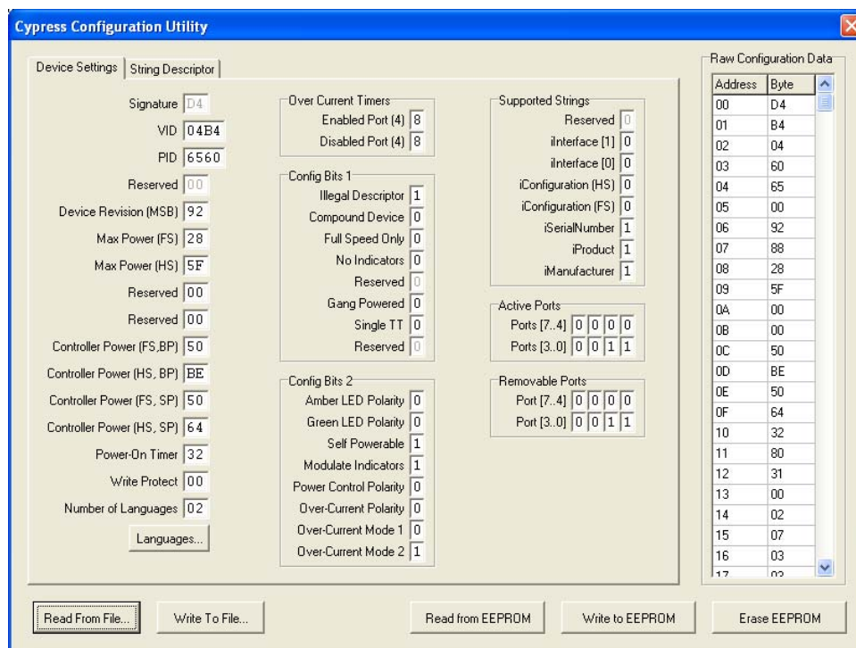
Figure 3-1. Configuration Utility
