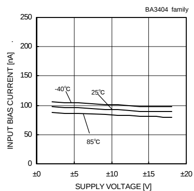
Fig. 105 Input Bias Current - Supply Voltage (Vicm=0[V], VOUT=0[V])
