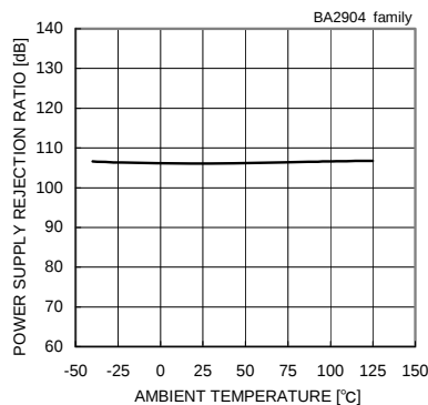
Fig. 72 Power Supply Rejection Ratio - Ambient Temperature
