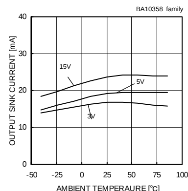
Fig. 9 Output Sink Current - Ambient Temperature ( V_{OUT}=V_{CC} )
