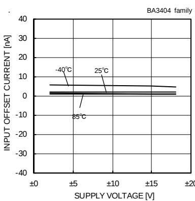
Fig. 107 Input Offset Current - Supply Voltage (Vicm=0[V], VOUT=0[V])
