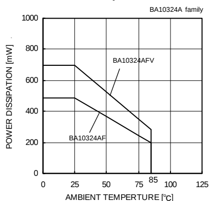
Fig. 25 Derating Curve
