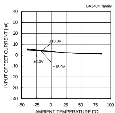
Fig. 108 Input Offset Current - Ambient Temperature (Vicm=0[V], VOUT=0[V])
