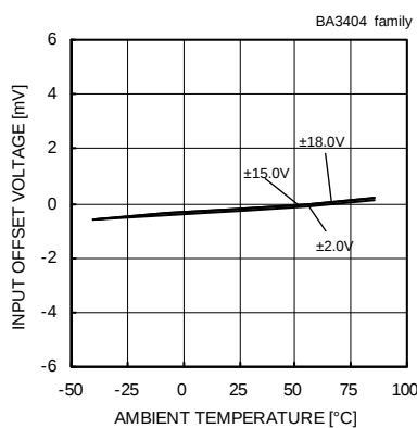
Fig. 104 Input Offset Voltage - Ambient Temperature (Vicm=0[V], VOUT=0[V])
