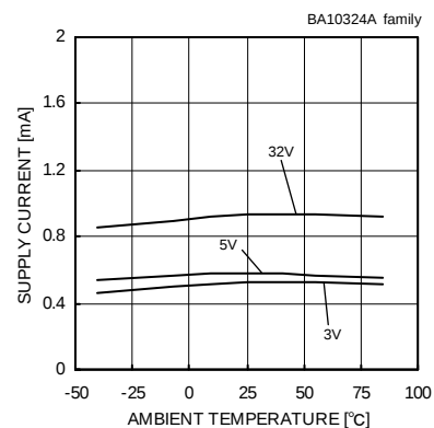
Fig. 27 Supply Current - Ambient Temperature
