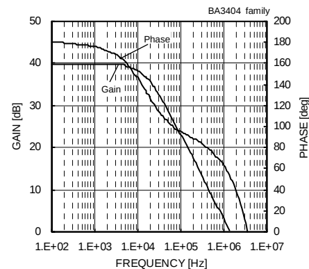
Fig. 114 Voltage Gain - Frequency (VCC=±15V)
