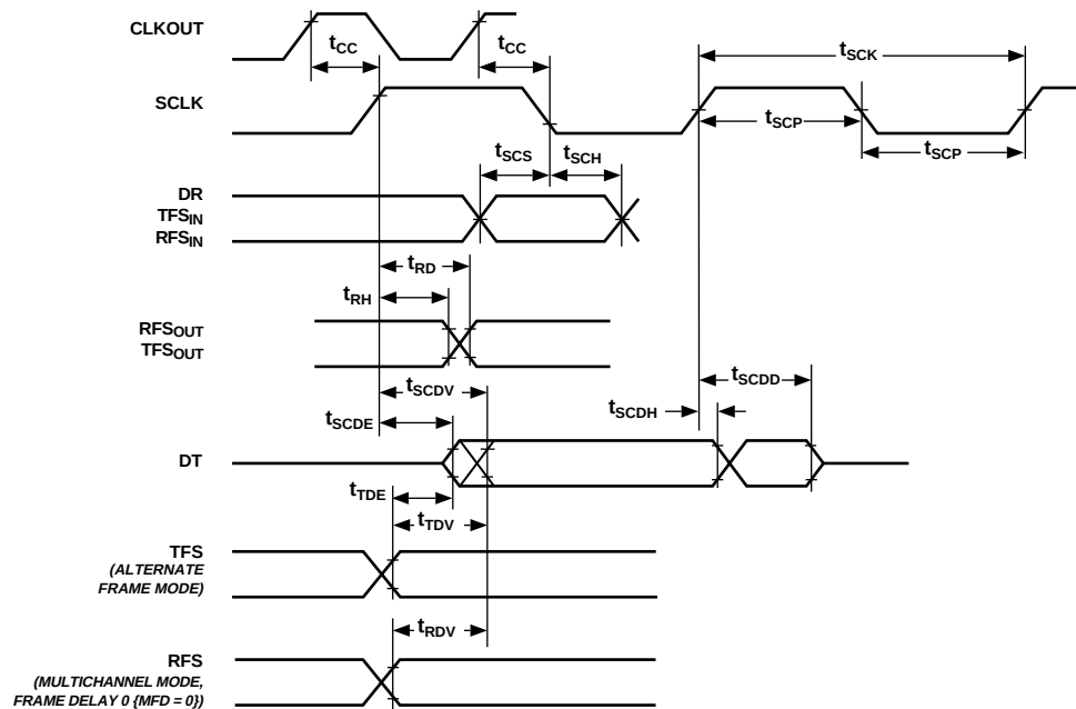
Figure 32. Serial Ports
