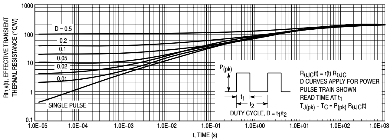
Figure 15. Thermal Response
