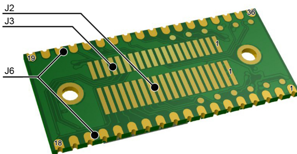
Figure 9: The solder pads J6 are available on the long edges of the bottom side of the PCB. The board-to-board connector pads J2-J3 are located between the mounting holes.
