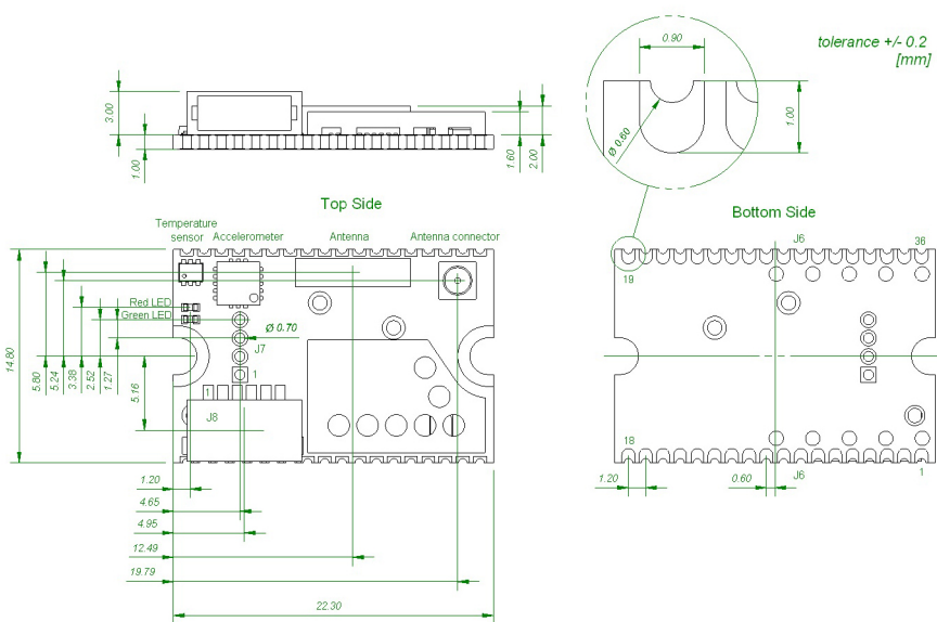
Figure 11: cB-OLP425 and cB-OLS425 module dimensions.
