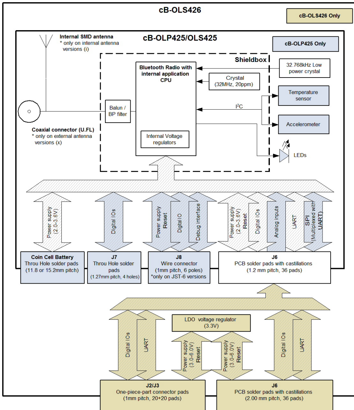
Figure 5: Block diagram of cB-OLP425/OLS425 and cB-OLS426. Notice that the Serial port Adapters (cB-OLS425/426) does not include all functions as the platform (cB-OLP425). The cB-OLS426 is a cB-OLS425 mounted on a carrier board with an LDO regulator.
