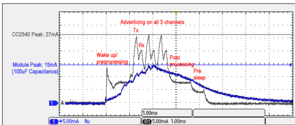
Figure 10: cB-OLS425 current consumption during advertising. The grey curve is moment radio consumption and the blue is smoothed-out because of the 100uF capacitance to offload the battery. An 10ohm resistance is used as internal power source resistance in the measurements. The energy consumption (mAh) is the integration (area under the curves) of the curves.
