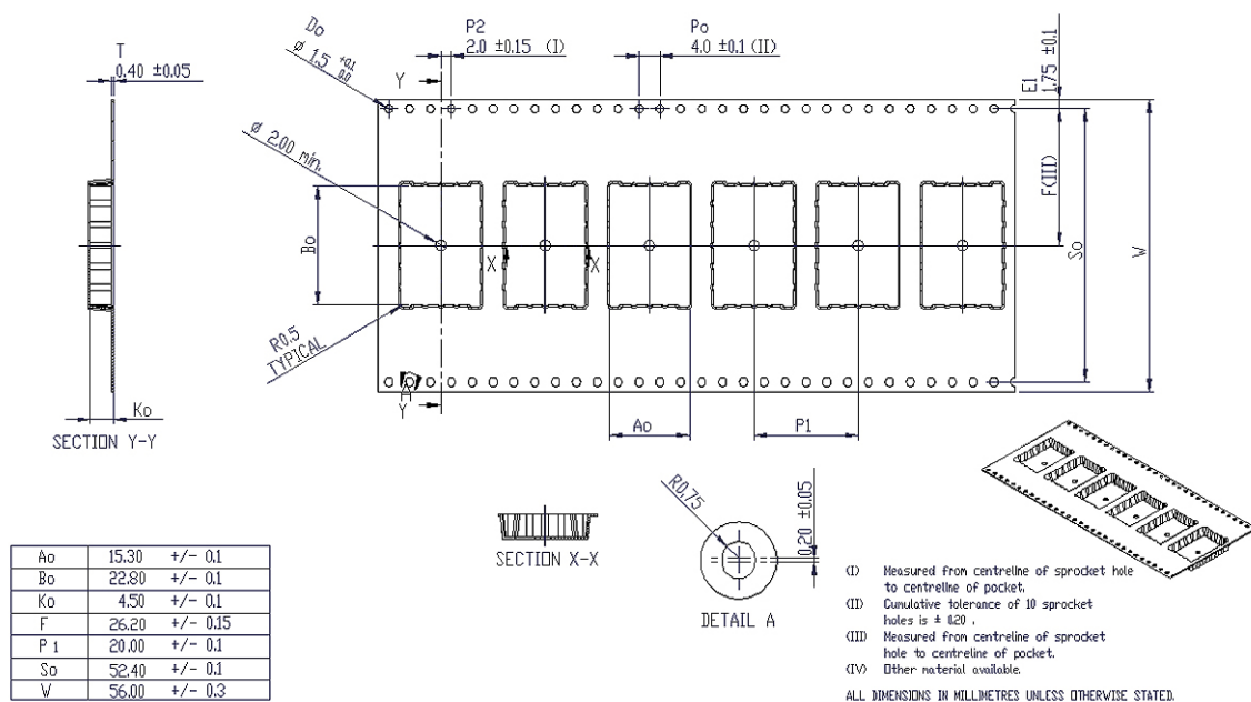
Figure 16: cB-OLP425 and cB-OLS425 tape dimensions.
