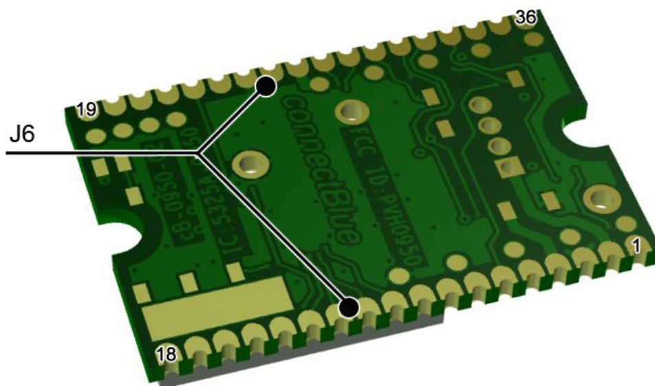
Figure 8: The solder pads J6 are available on the long edges of the bottom side of the PCB.
