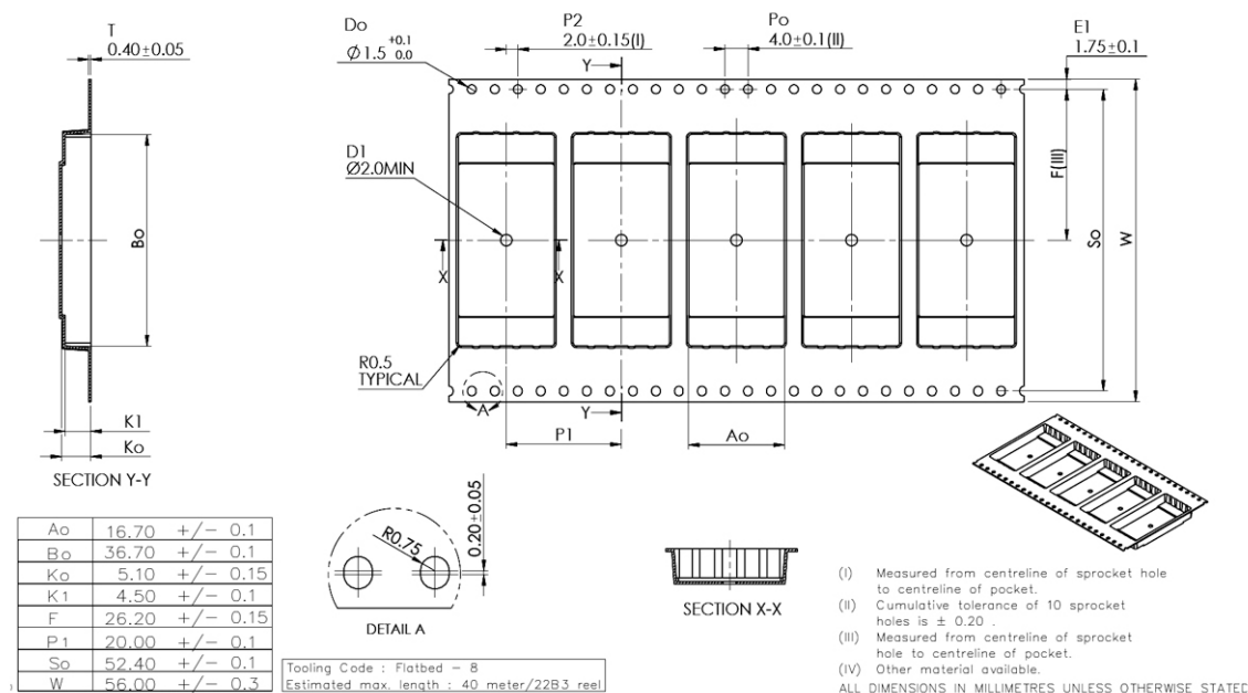
Figure 17: cB-OLS426 tape dimensions.
