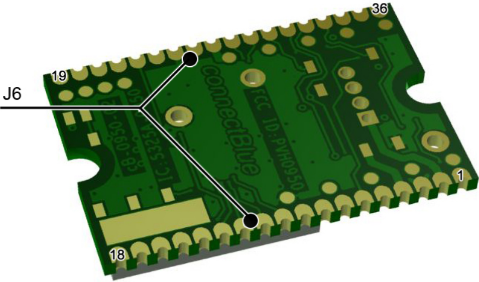
Figure 6: The solder pads J6 are available on the long edges of the bottom side of the PCB.
