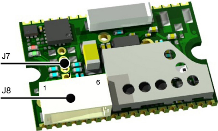
Figure 7: 4x1 through holes row J7 and the JST connector J8 mounted on the component side of the PCB.
