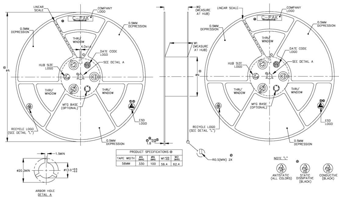
Figure 18: Tape real dimensions.
