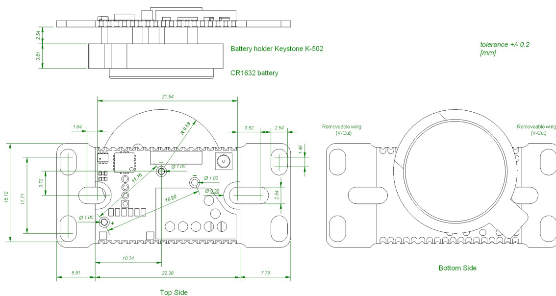
Figure 12: cB-OLP425 dimensions with mounting wings (optional) and CR1632 battery holder.
