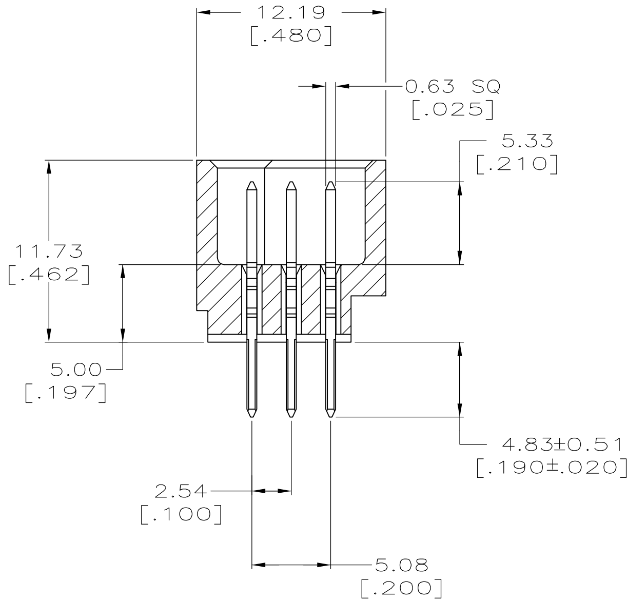
SECTION Z-Z
