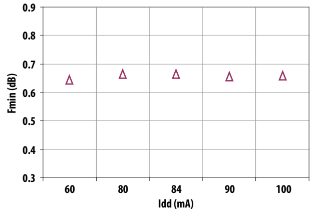
Figure 8. F_{min} vs I_{DD} at 4.8 V at 2 GHz
