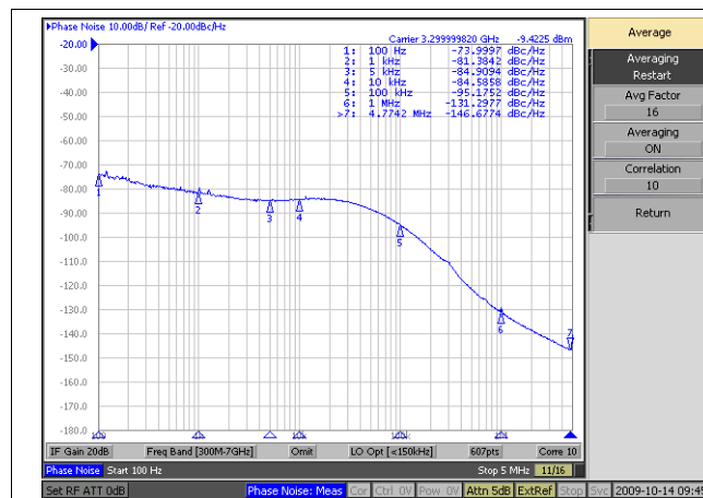
Figure 34. Phase Noise
