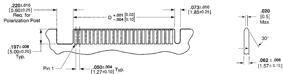
Recommended PC Board Layout for Card-edge Applications
