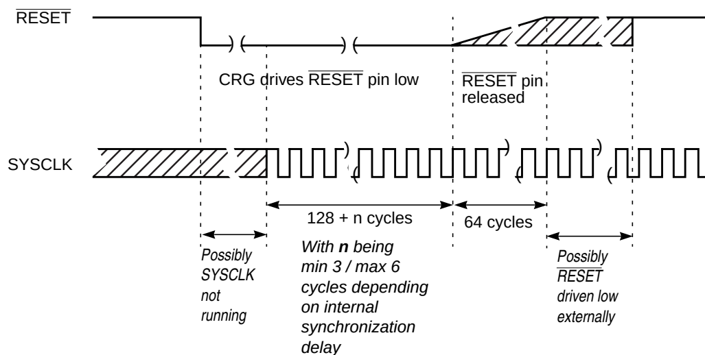
Figure 2-25. RESET Timing
