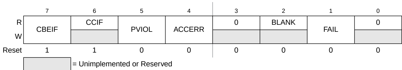
Figure 28-13. Flash Status Register (FSTAT — Special Mode)
