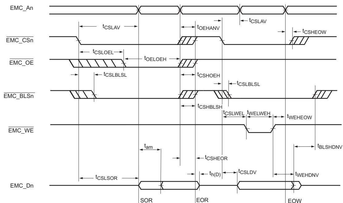
Fig 34. External static memory read/write access (PB = 1)
