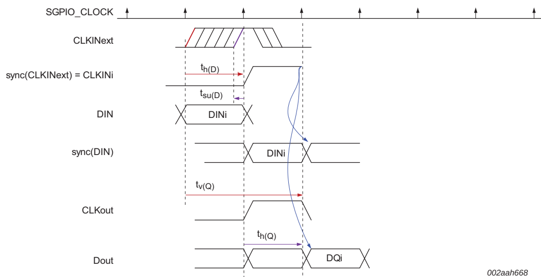
Fig 32. SGPIO timing
