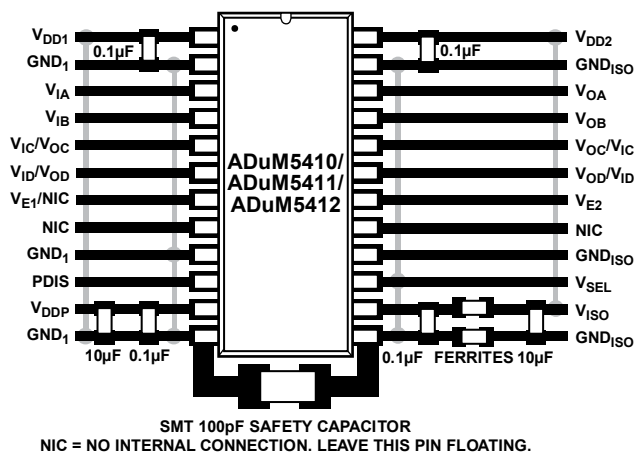
Figure 32. Recommended PCB Layout
