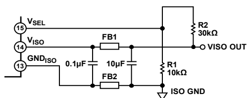
Figure 31. V_{\text{ISO}} Bias and Bypass Components
