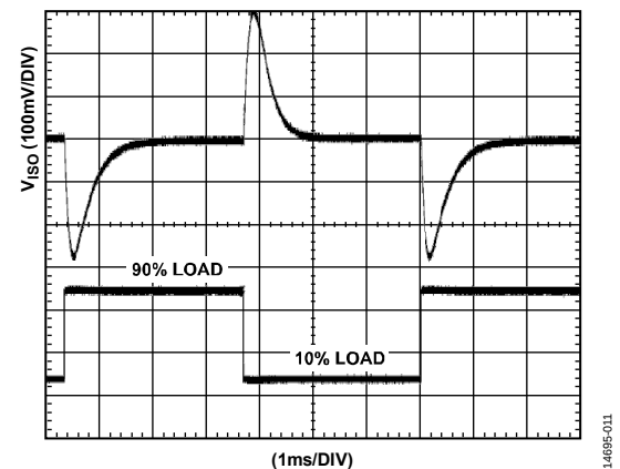
Figure 10. V_{ISO} Transient Load Response, 5 V Output, 10% to 90% Load Step
