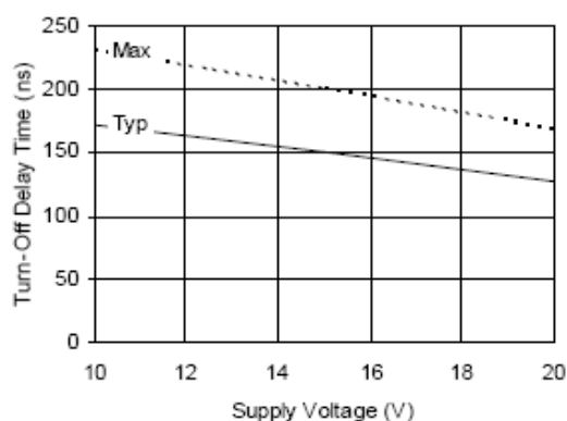
Figure 7B. Turn-Off Propagation Delay vs. Supply Voltage
