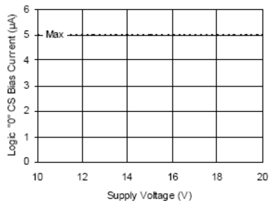
Figure 21B. Logic "0" CS bias current vs. Voltage
