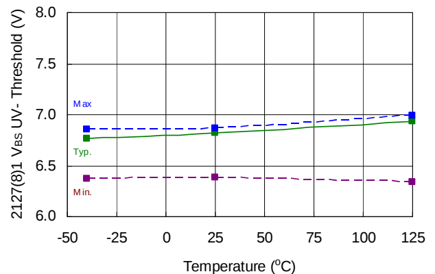
Figure 22B. 2127(8)1 V_{BS} UV threshold - vs. Temperature
