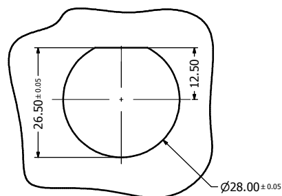
Recommended Panel Cutout (e)
