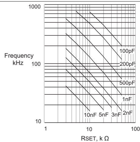
Figure 11. Oscillator Frequency vs R_{\text{SET}} and C_T
