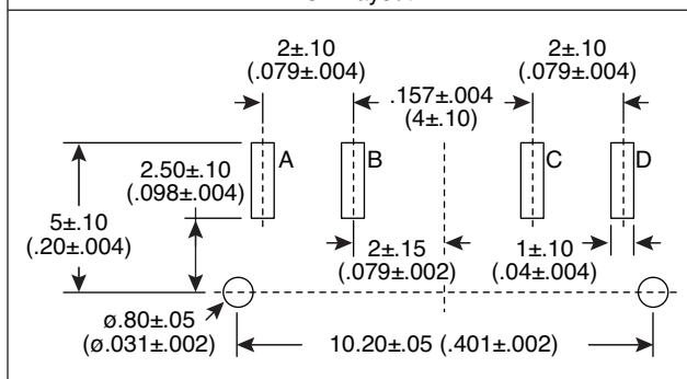
PCB Layout
