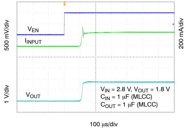
Figure 29. Enable Turn-on Response – C_{OUT} = 1\text{ μF} , I_{OUT} = 250\text{ mA}
