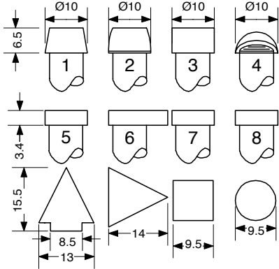
lenses 1-2 standard
