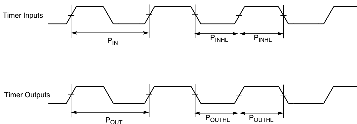
Figure 36. Timer Timing
