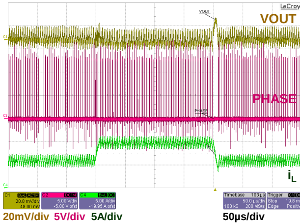
Figure 15: Load Transient 6-10A
